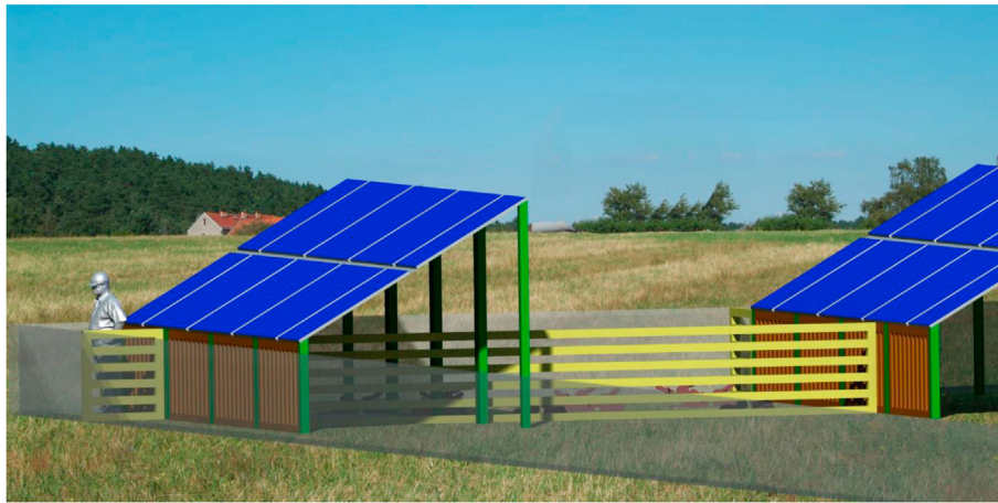
Fig. 3. Front side of cutaway section of rabbit agrivoltaic sections showing permanent fences (clear for exterior and brown for rack fences) as well as movable fences yellow. (For interpretation of the references to colour in this figure legend, the reader is referred to the Web version of this article.)
