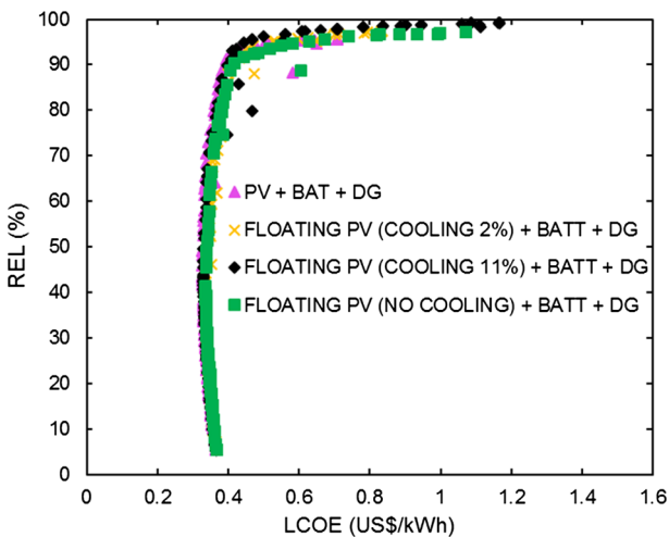
Fig. 11. Pareto front for the ground mounted and floating PV hybrid energy system.
