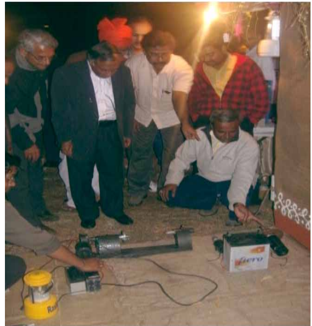
A hut demonstrating solar powered textile unit
