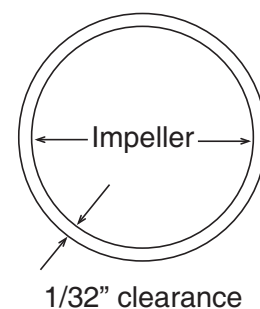
Figure 5. Impeller Eye and Wear Ring
