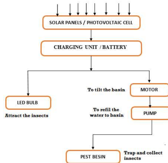
Fig -1: Schematic representation of solar insect trap
