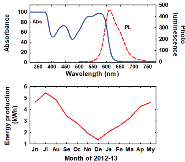
Figure 3. (Top) Dye absorption spectrum (Abs, solid line) and photoluminescence emission spectrum (PL, dashed line) for dye in polymethyl methacrylate (PMMA). (Bottom) Monthly energy production of a single panel in glasshouse with Wavelength Selective Photovoltaic (WSPV) roof.
