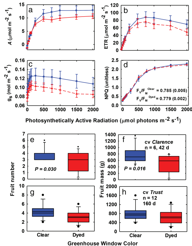
Figure 4. Photosynthesis and development of tomatoes grown under WSPVs and clear greenhouse windows. (A) Photosynthetic CO 2 assimilation (A, \mu\text{mol CO}_2 \text{ m}^{-2} \text{ s}^{-1} ) as a function of photosynthetically active radiation (PAR; 400–700 nm). A PAR of 2000 \mu\text{mol photons m}^{-2} \text{ s}^{-1} is roughly equivalent to full sun in the temperate zone at noon in early summer. (B) The rate of electron transport (ETR, \mu\text{mol electrons m}^{-2} \text{ s}^{-1} ) through PSII in chloroplasts, which links the light reactions with CO 2 fixation into sugars. (C) Stomatal conductance to water vapor ( g_s , \text{mol H}_2\text{O m}^{-2} \text{ s}^{-1} ) in response to PAR, an indication of water use by leaves. (D) Nonphotochemical quenching (NPQ, unitless) in response to PAR, reflecting in part photoprotective energy dissipation. Blue solid lines are for plants under clear PMMA plastic and red dashed lines are for plants under luminescent-dyed PMMA. Data are means \pm SE ( n = 6 ). Panels E–H: Total number fruit per plant (E, G) and mass of fruit per plant (F, H) for tomato ( Lycopersicon esculentum cv Clarence (E, F) and cv Trust (G, H)) grown under clear plastic or red luminescent dye in plastic (PMMA). Data are means (horizontal black line), standard error (wide colored bars), standard deviation (whiskers) and outliers (points) for the number of plants and time duration shown. Blue bars correspond to plants under clear PMMA and red bars are for plants under dye in PMMA.
