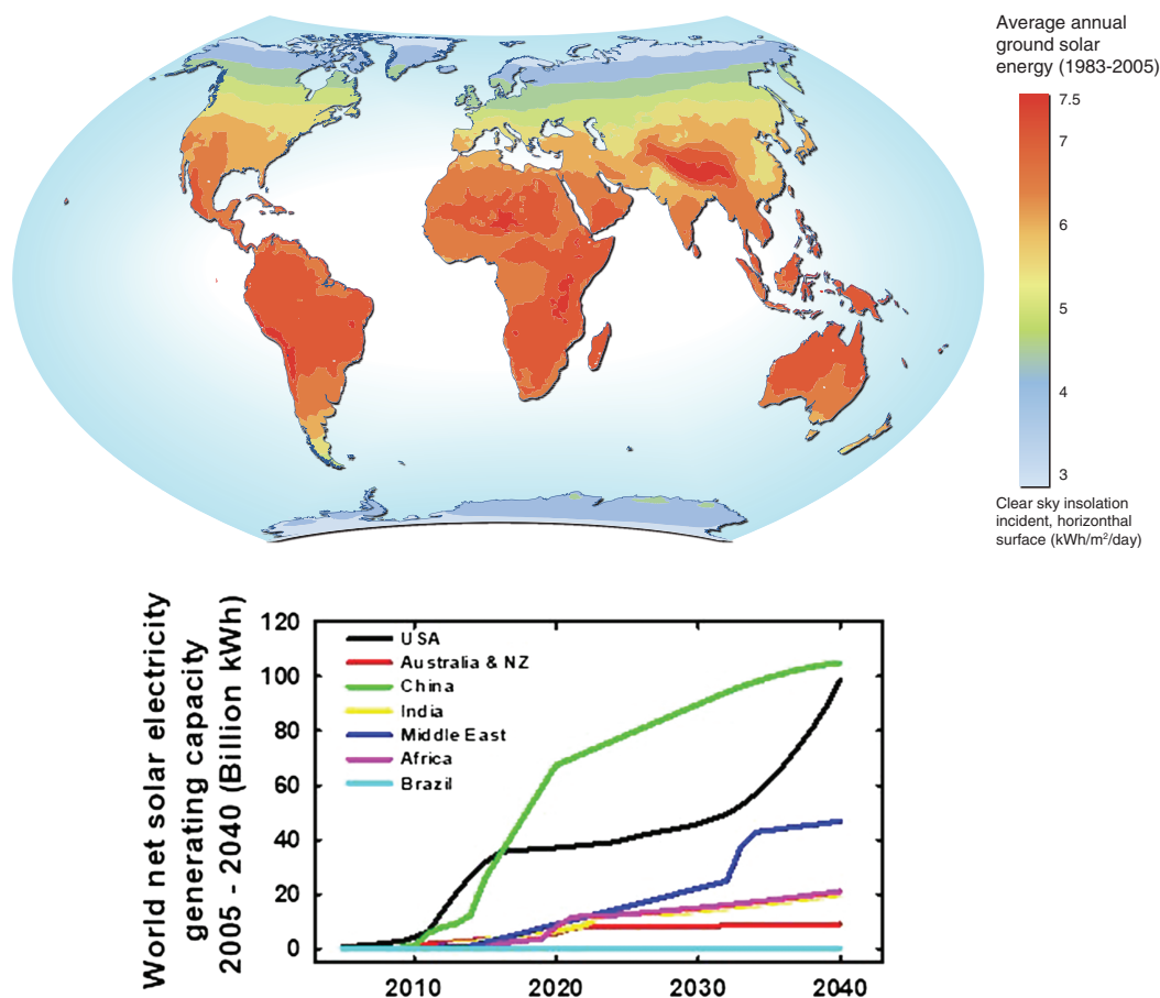
Figure 1. Average global distribution of surface solar radiation interception for the period 1983–2005 (top). Image source: UNEP/GRID-Arendal ( http://www.grida.no/graphicslib/detail/natural-resource-solar-power-potential_b1d5 ), courtesy of Hugo Ahlenius. Bottom: Projected global electricity generation potential for the period 2005–2040. Source: U.S. Energy Information Agency (July 2013).
